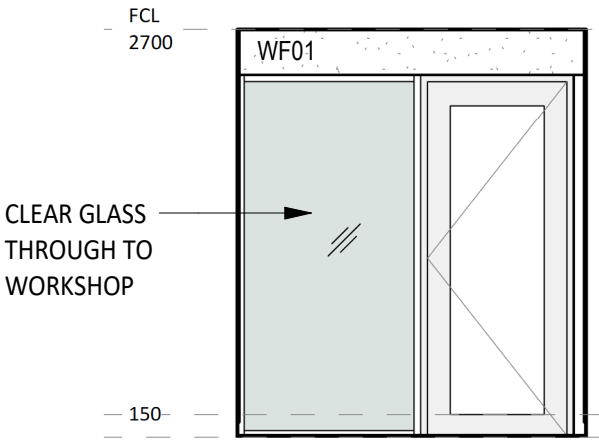
5 ELEVATION DETAIL 60-007 1 : 50
