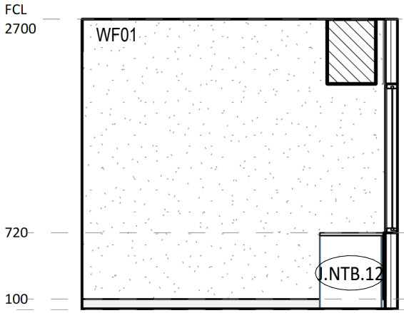
2 ELEVATION DETAIL 60-007 1 : 50
