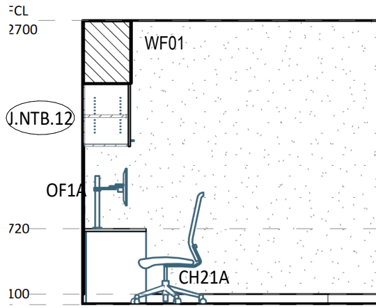
4 ELEVATION DETAIL 60-007 1 : 50
