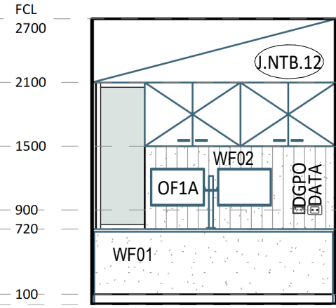
3 ELEVATION DETAIL 60-007 1 : 50
